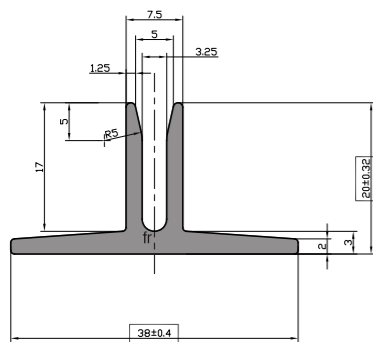
13. Large D Tee - GPM10905
