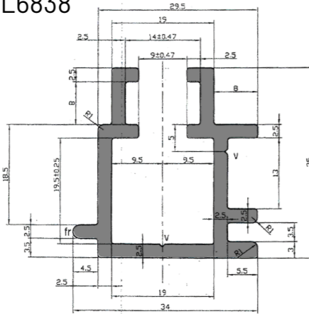
8. Large Interlock Light - YL6838
