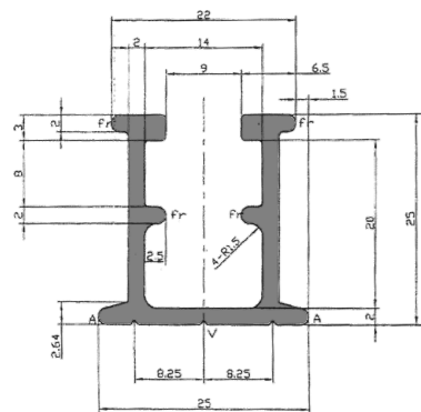
13. Large D Tee - GPM10905
