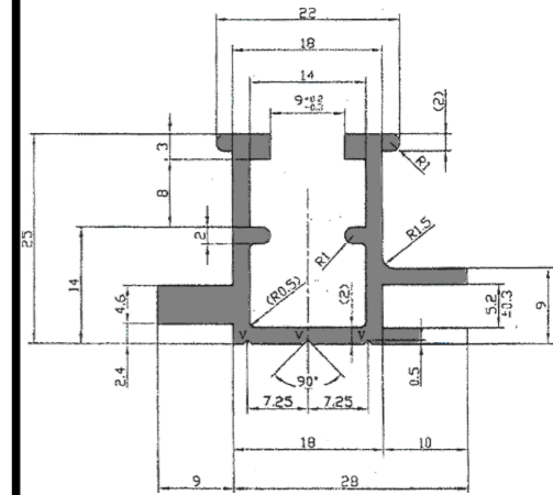
6. Medium Interlock Heavy - YL6841
