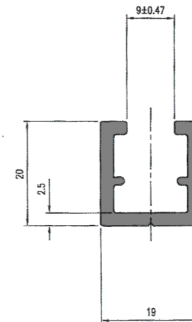
11. Large Heavy - GBH0009
