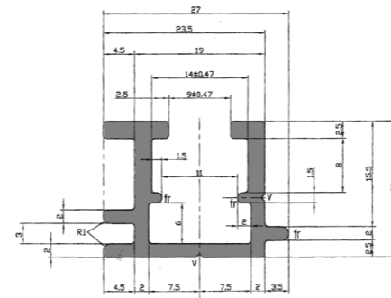
4. Medium Interlock Light - YL6837
