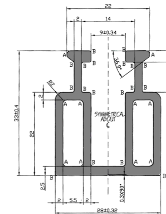
11. Large Heavy - GBH0009
