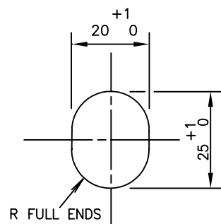
DETAIL OF SLOT (4 POSNS)
