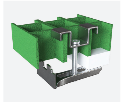
J Clamp
